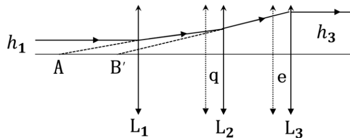
Figure 8. Principle Diagram of the Afocal Zoom Beam Expander System
