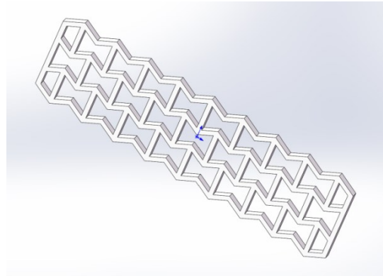
Figure 2. The 3D design drawing of Negative Poisson's ratio structure in Solidworks
