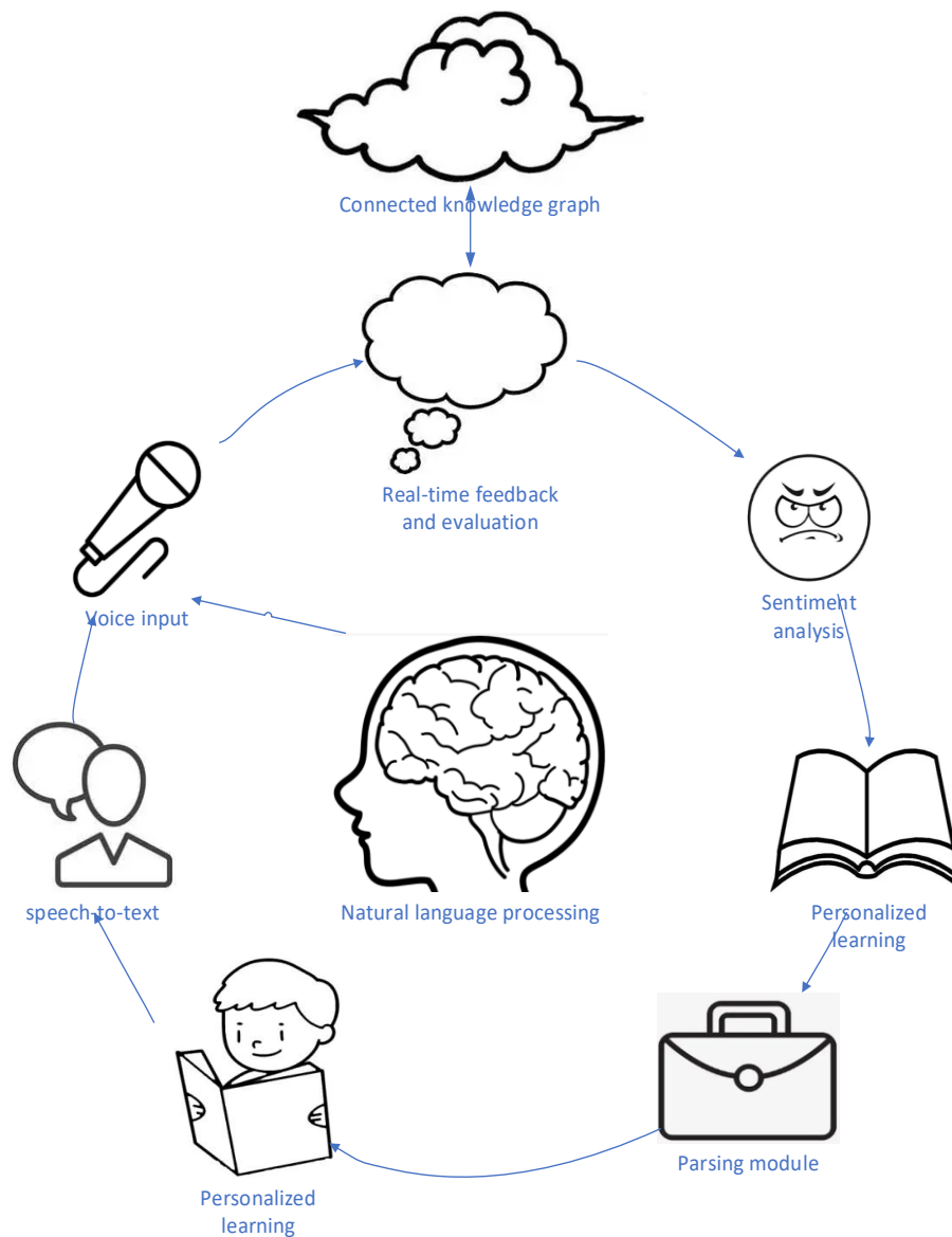
Figure 2. System Framework
