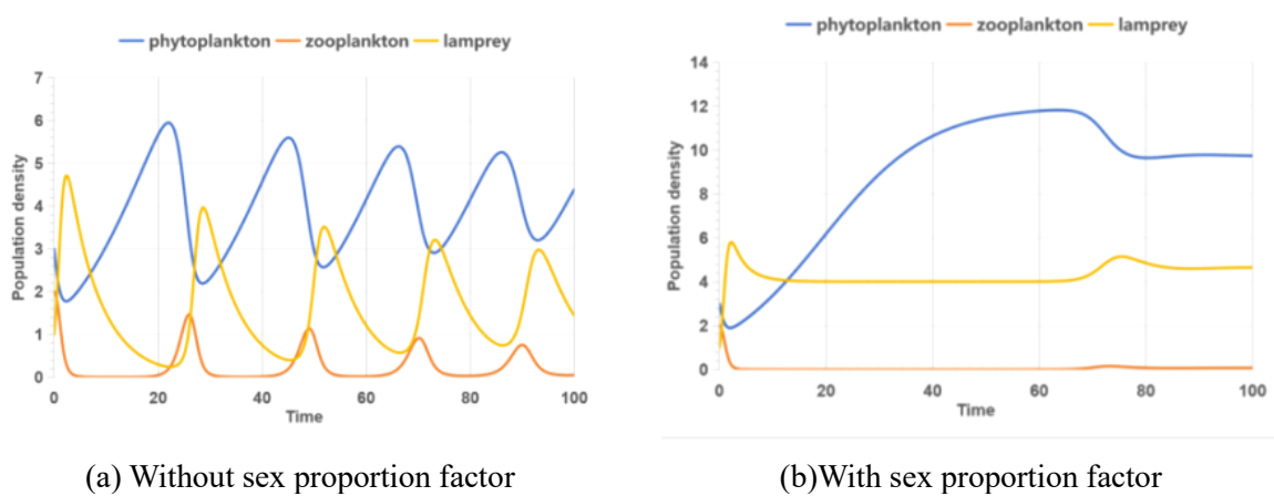
Figure 3. Population density - time curve
