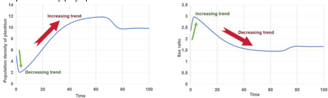
(a) Change in population density of planktonic organisms
